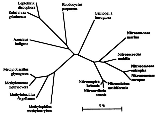
FIG. 3. Distance tree for the beta subdivision of the proteobacteria.
