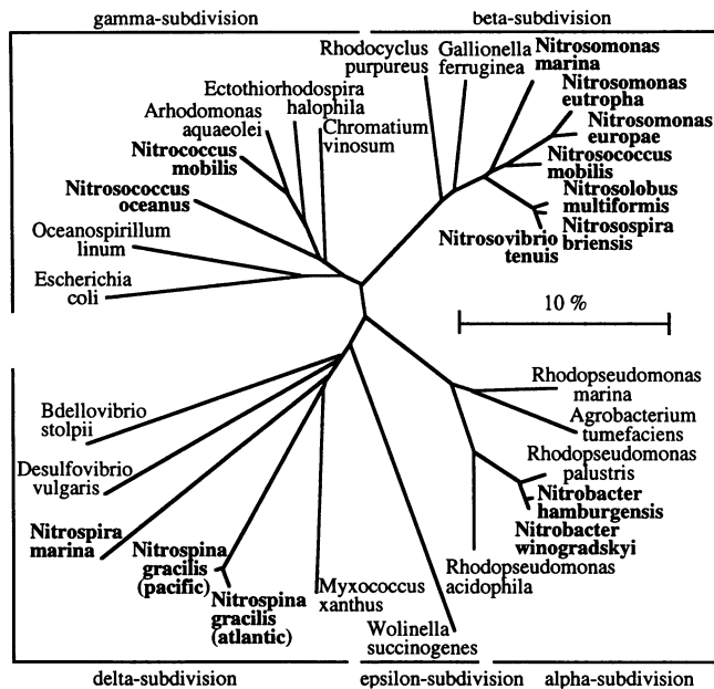
FIG. 1. Distance tree for the the proteobacteria, including the nitrifying isolates characterized in this study. The scale bar corresponds to 0.1 estimated fixed mutation per sequence position.
