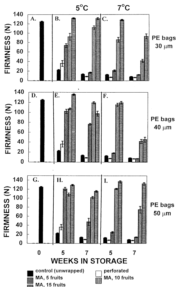
Fig. 2. Effect of storage temperature, bag thickness and number of fruit in the bag on the firmness of 'Hass' avocado fruit immediately after 5 or 7 weeks of storage. Values represent means \pm SE of 20 determinations of 10 fruit (Exp. 1).
