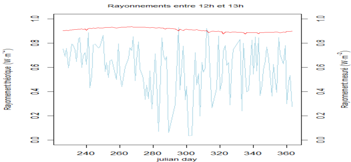
Figure 14: Rayonnement (12-13h) 2011
