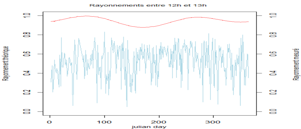
Figure 15: Rayonnement (12-13h) 2012
