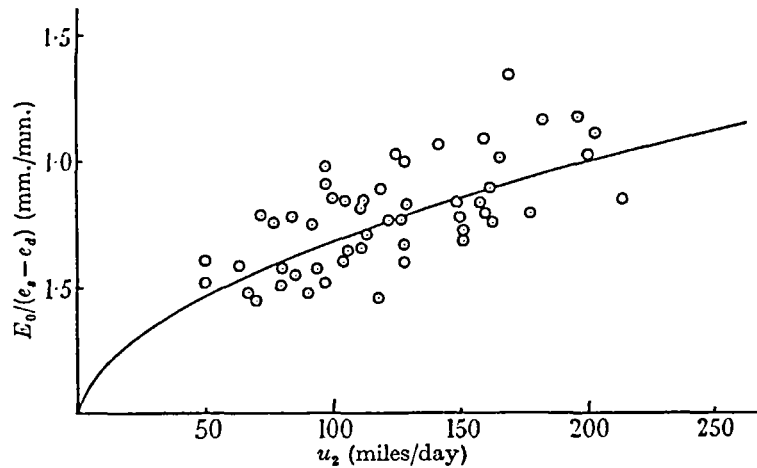
FIGURE 3. Daily evaporation per unit partial pressure difference for open water surface (tank MO). The curve is: E_0/(e_s - e_d) = 0.065 u_2^{0.64} .
