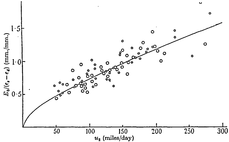
FIGURE 2. Daily evaporation per unit partial pressure difference for open water surface (cylinder O). The curve is: E_0/(e_s - e_d) = 0.033 u_2^{0.68} , \circ 1944, \bigcirc 1945.
