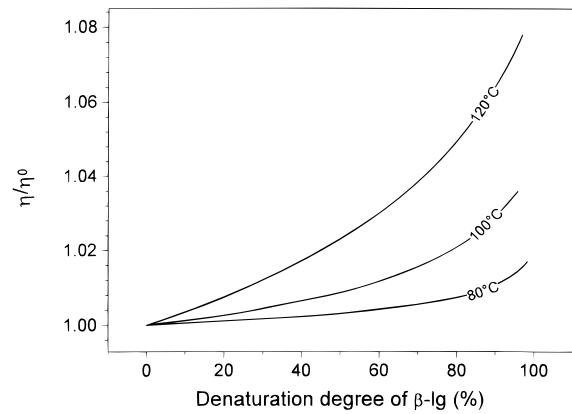
Figure 6. Viscosity change of skim milk as a function of the heating temperature and the degree of \beta -lactoglobulin denaturation (model simulations). The heating time was adjusted for the given denaturation degree and heating temperature.
