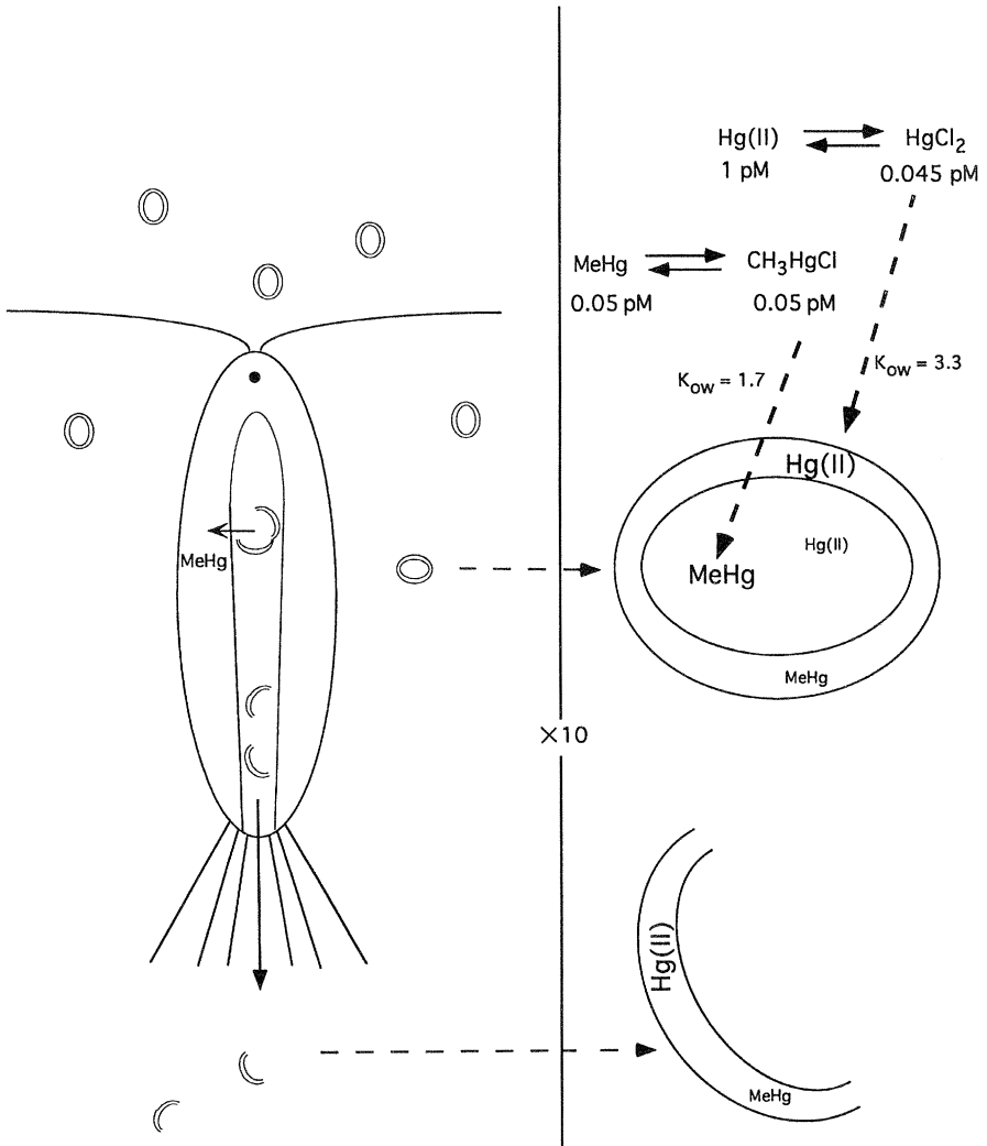
Figure 8 Bioaccumulation of mercury in the first steps of the food chain. \text{Hg(II)} and \text{MeHg} concentrations are estimates for average seawater (27); \text{HgCl}_2 and \text{CH}_3\text{HgCl} concentrations are calculated (see Table 1). See text for explanations.
