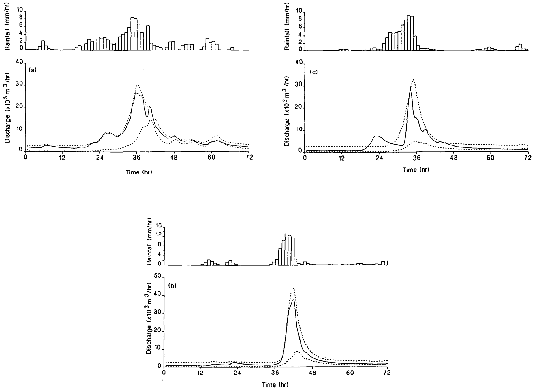
Figure 9. Predictive uncertainty for three storms based on a priori parameter distribution. Solid line indicates observed flow, dashed line indicates 5 and 95 per cent simulation limits. (a) Storm 6. (b) Storm 8. (c) Storm 9
