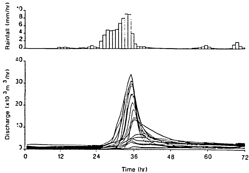
Figure 3. A subset of 20 simulations for storm 1
