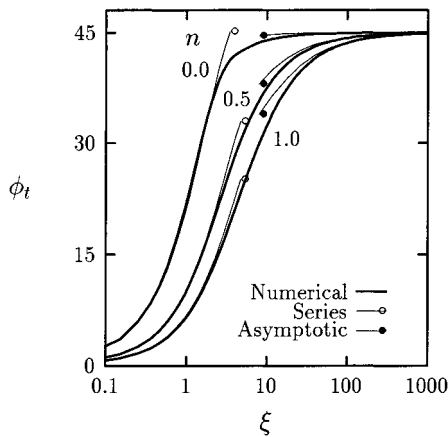
Figure 2. Phase angle of rate of heat transfer for different values of n .
