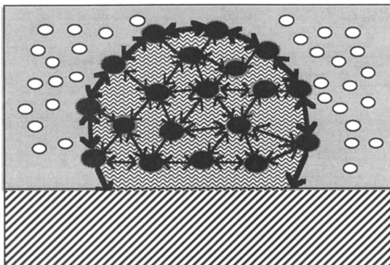
Fig. 1. Illustration of surface tension arising from the imbalance of molecular attraction forces in a liquid drop (adapted from Weber, 1972).
