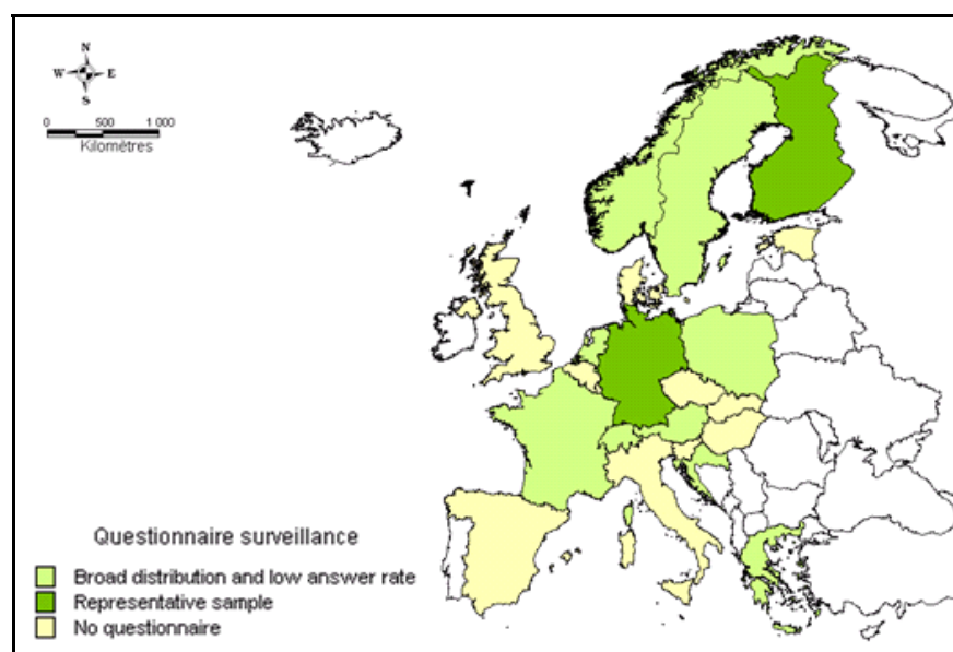
Figure 22. Questionnaire surveillance in Europe
